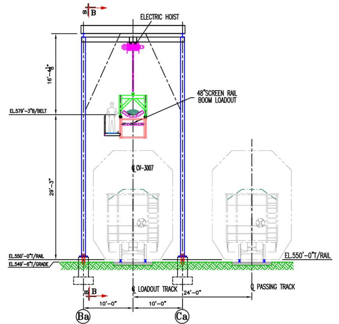
SECTION E-E
